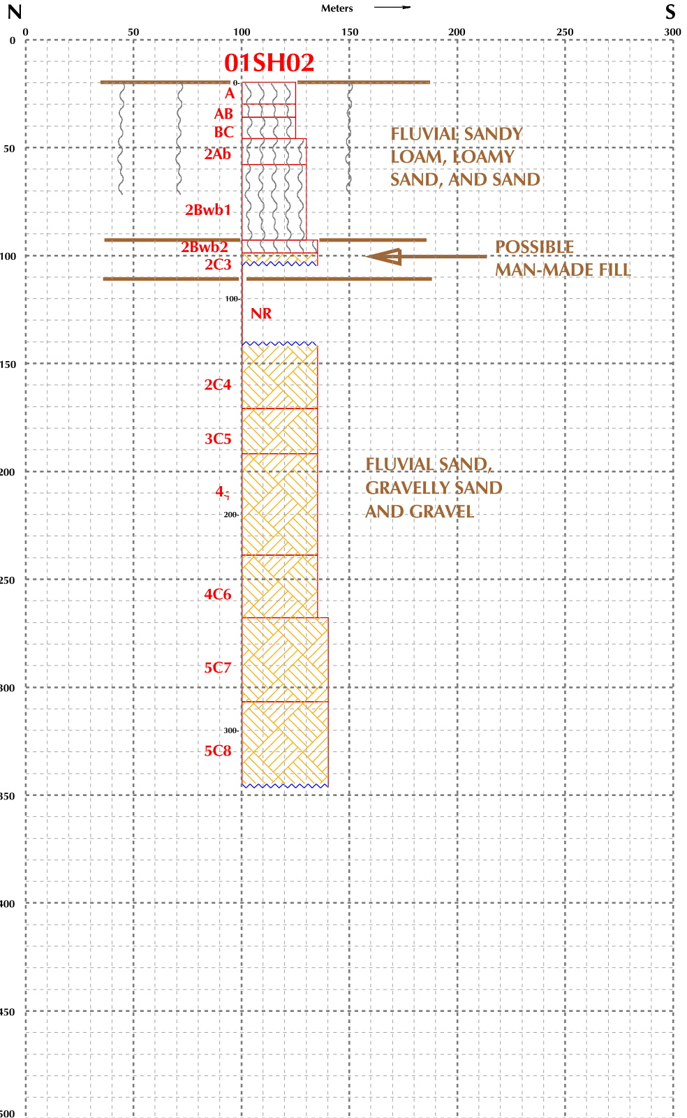
FIGURE 25 GRAPHIC SEDIMENT/ SOIL LOG OF THE FFW LANDFORM SEDIMENT ASSEMBLAGE AT CORE LOCATION 01SH02
