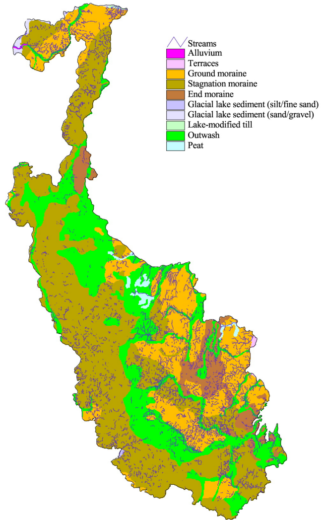
Generalized Quaternary Geology
